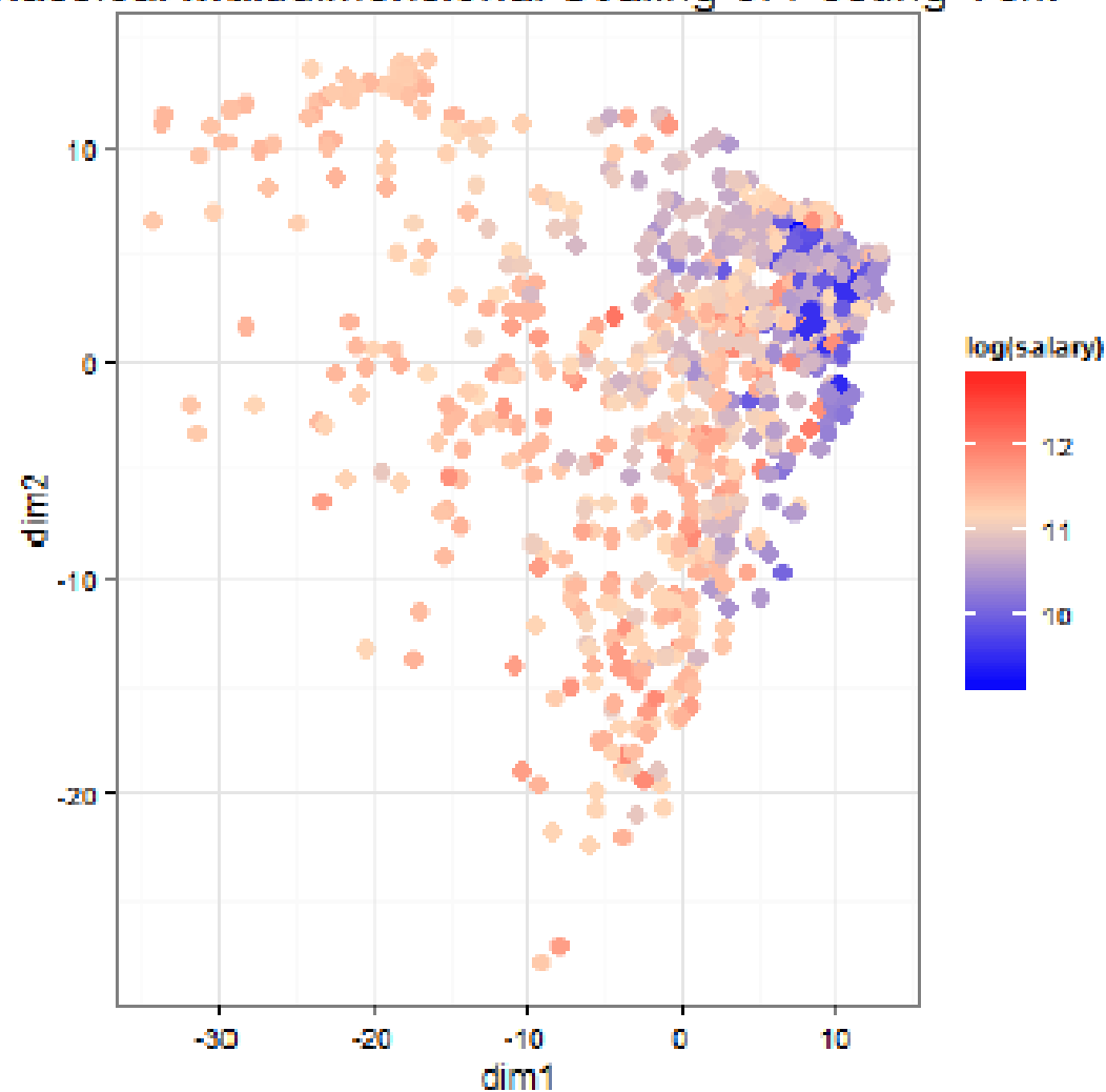
Classical Multidimensional Scaling of Posting Text
