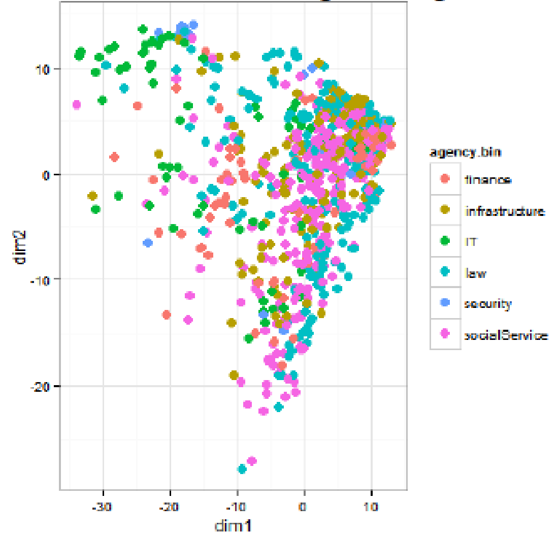
Classical Multidimensional Scaling of Posting Text
