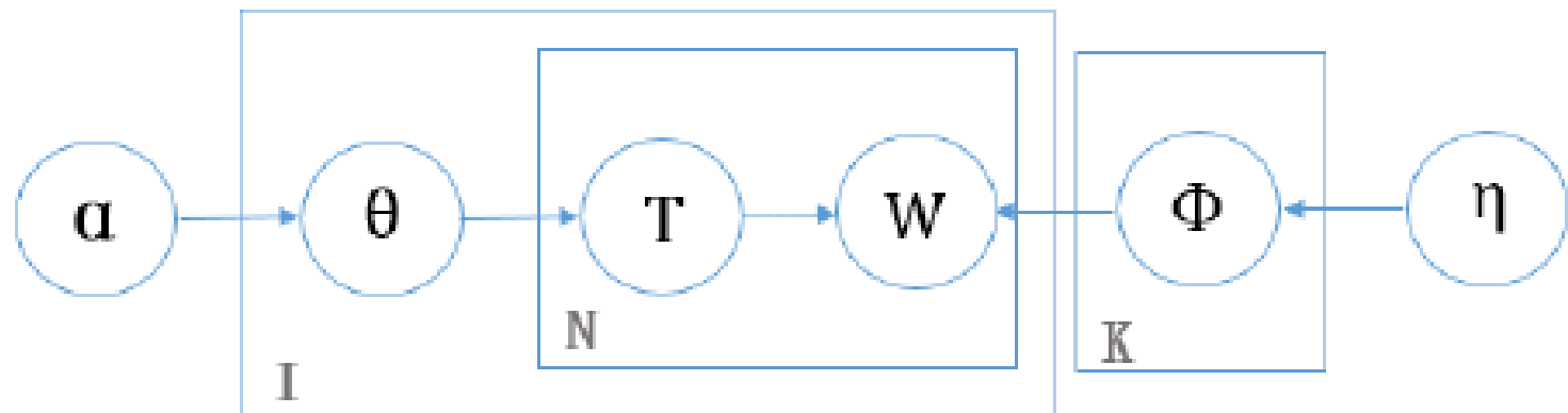
Plate Diagram for Latent Dirichlet Allocation
