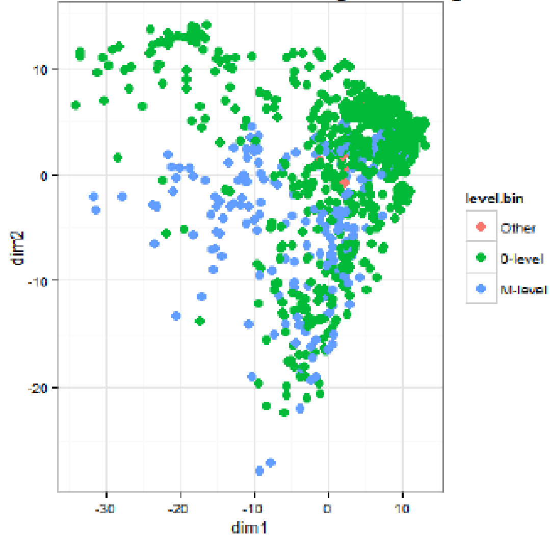
Classical Multidimensional Scaling of Posting Text
